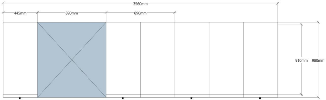
Top View
